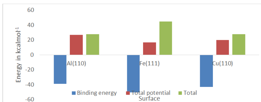
Figure 4: Binding energy, total potential energy of molecule, and total energy of amoxicillin on the surface of metal (Fe, Al, and Cu).
