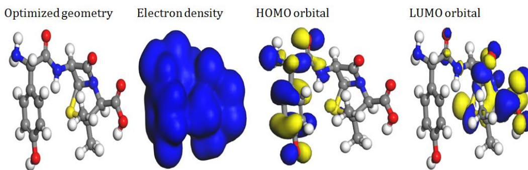
Figure 1: Optimization geometry, Electron density, HOMO, and LUMO orbitals of amoxicillin.
