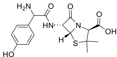
Scheme 1: Structure of amoxicillin.
