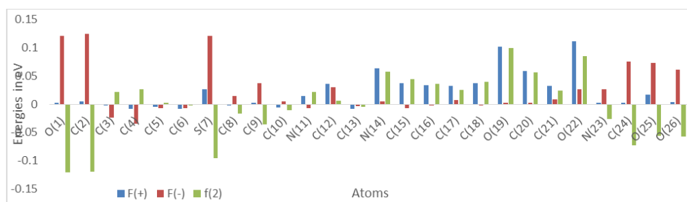
Figure 2: Graphical representation of Fukui values and Fukui second function.
